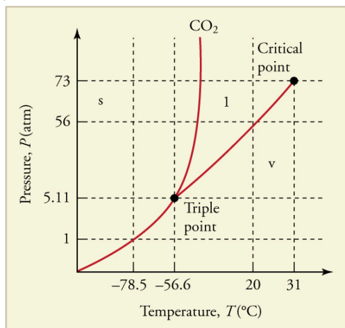
Figure 13.35 The phase diagram for carbon dioxide. The axes are nonlinear, and the graph is not to scale. Dry ice is solid carbon dioxide and has a sublimation temperature of -78.5^{\circ}\text{C} .
